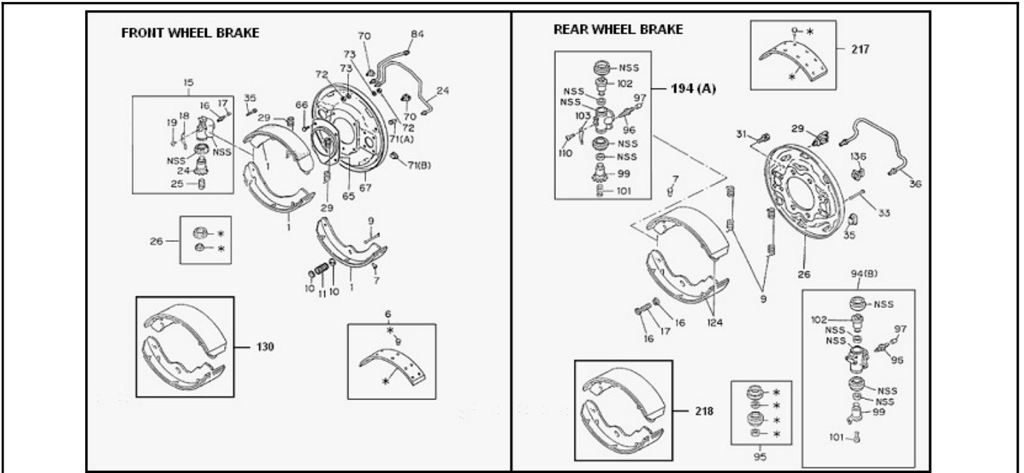
FIG.NO : 3-01 & 3-05 BRAKE SHOE FRONT & REAR
