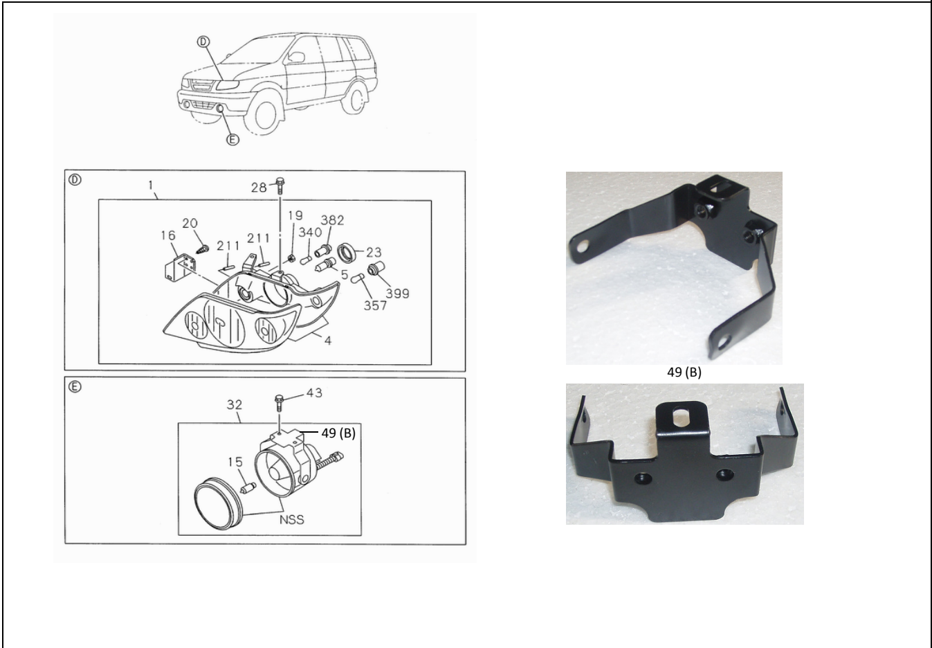
FIG NO: 8-01 LAMP; FRONT AND FRONT SIDE
