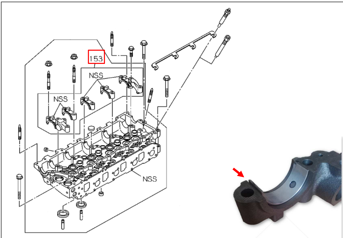
FIG NO : 0-11 CYLINDER HEAD
