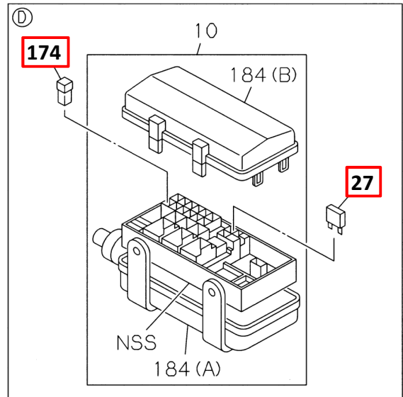
FUSE SLOW BLOW
