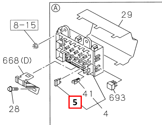
FIG.NO : 8-10 WIRING HARNESS AND FUSE
