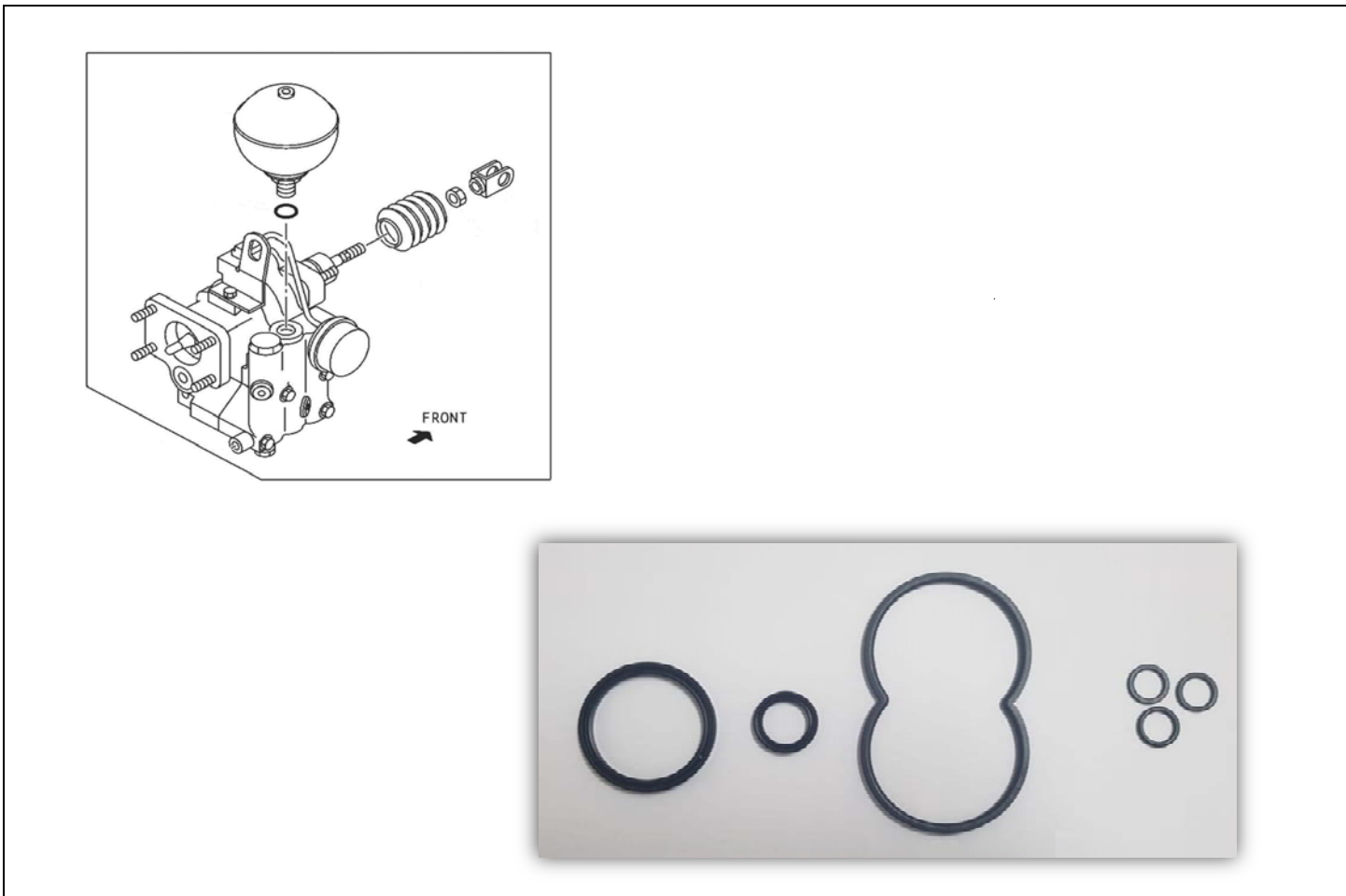
FIG NO : 3-31 BRAKE MASTER VAC AND BRAKE BOOSTER
