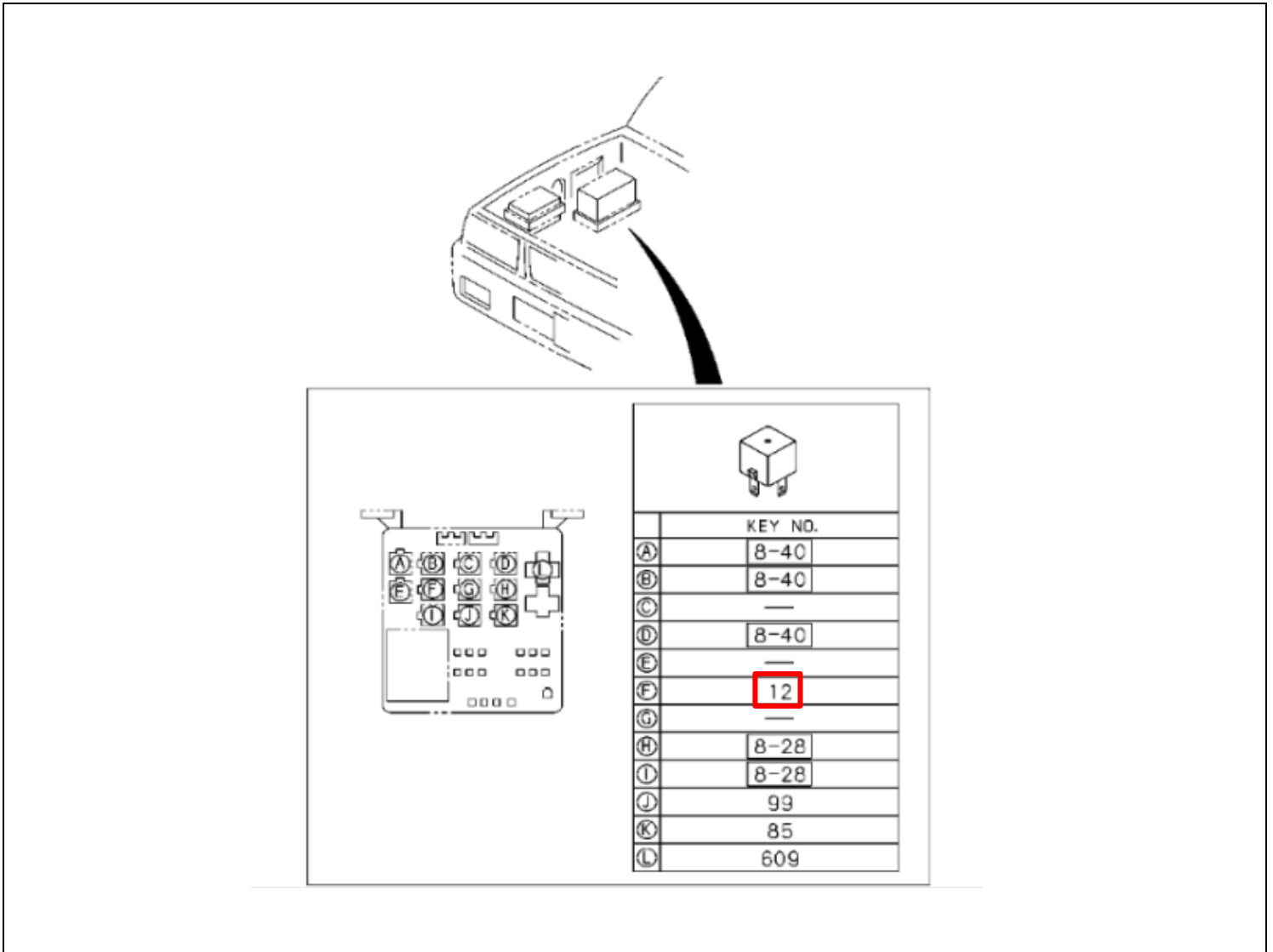
FIG NO : 8-25 SWITCH AND RELAY; INSTRUMENT PANEL
