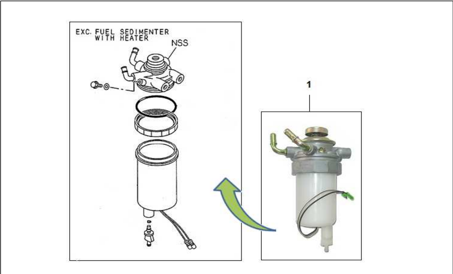
FIG.NO : 1-45 WATER SEDIMENTER FUEL
