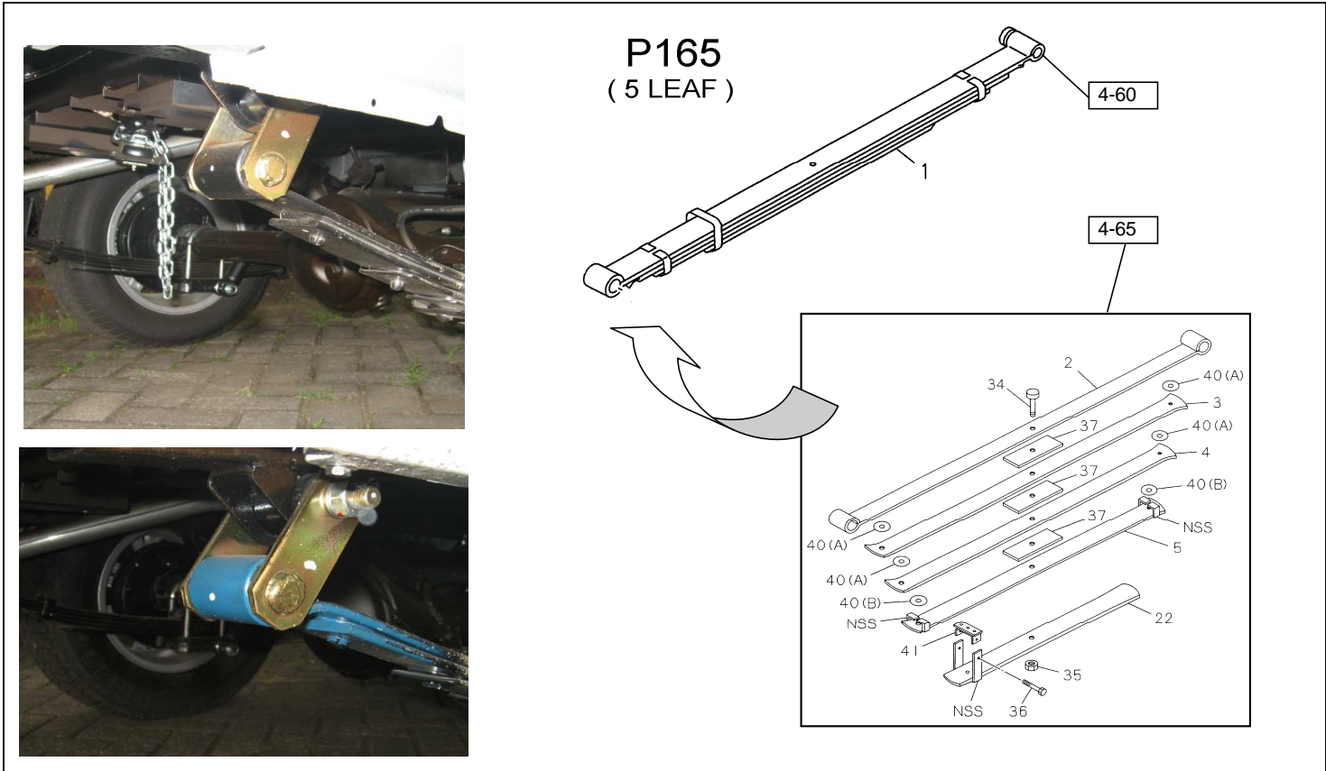
FIG.NO : 4-60 REAR SUSPENSION & 4-65 REAR LEAF SPRING
