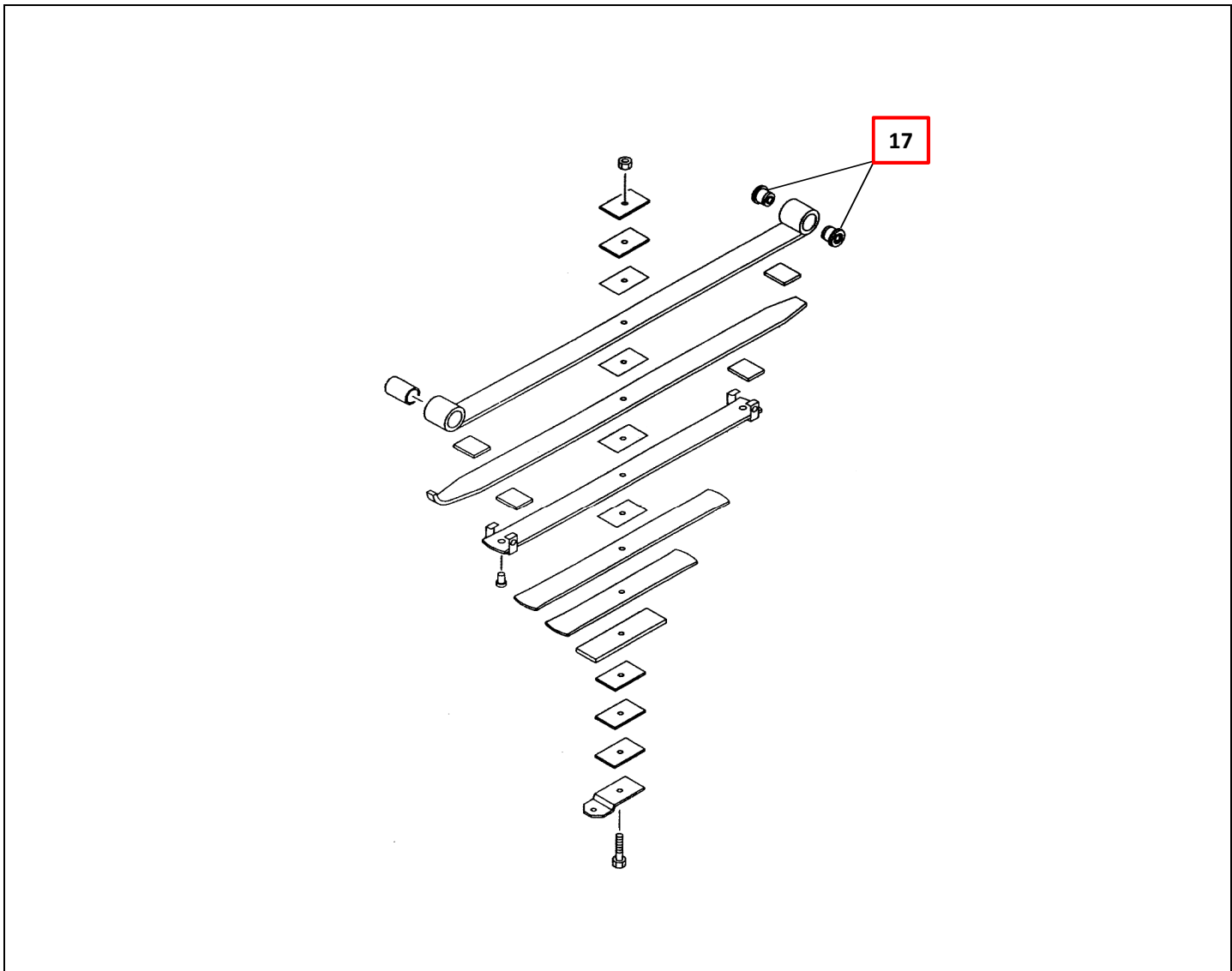
FIG.NO : 4-55 FRONT LEAF SPRING
