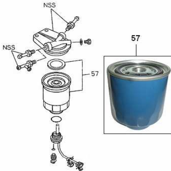
FIG.NO : 1-45 WATER SEDIMENTER FUEL
