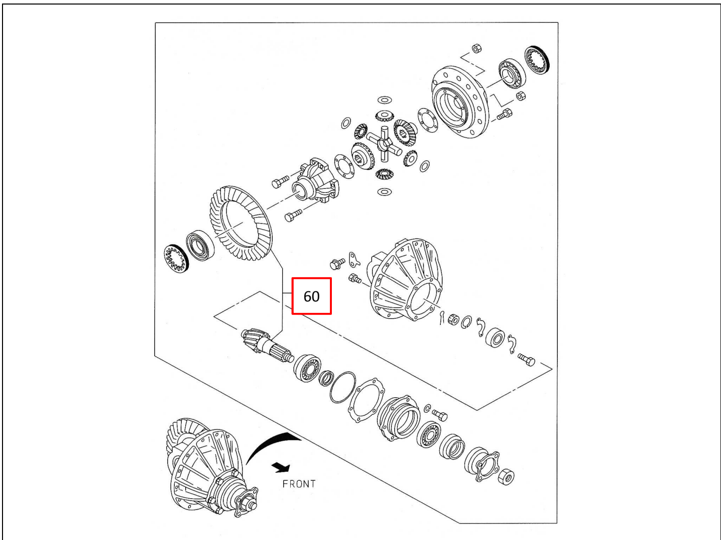
FIG NO : 4-25 REAR FINAL DRIVE
