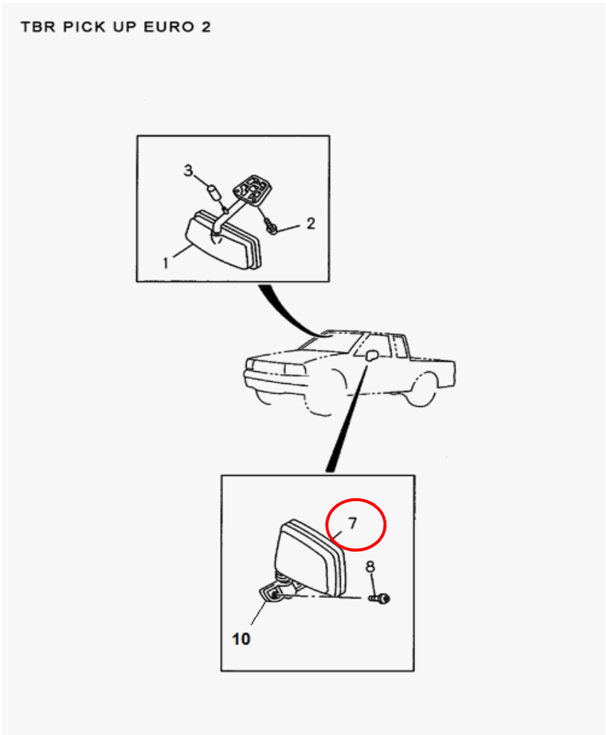
FIG NO : 7-20 MIRROR AND MIRROR STAY
