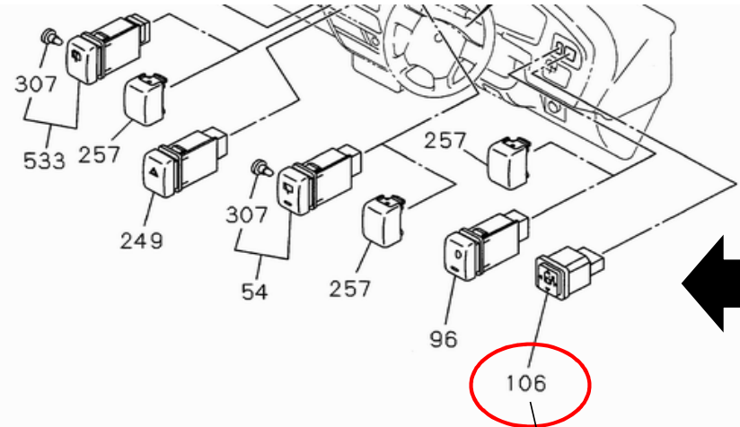
FIG.NO : 8-25 SWITCH AND RELAY; INSTRUMENT PANEL
