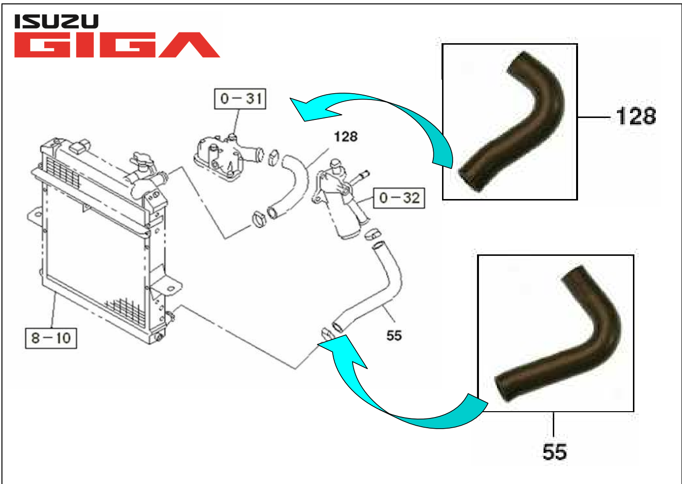
FIG.NO : 1-11 RADIATOR HOSE AND SUB TANK
