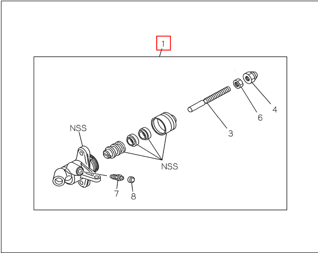
FIG NO : 2-06 CLUTCH SLAVE CYLINDER
