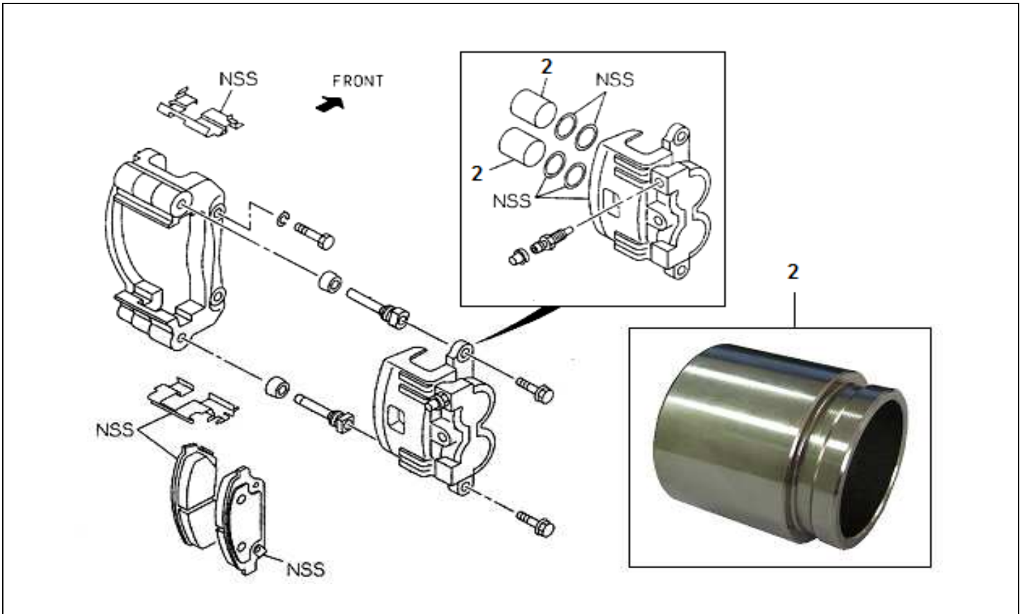
FIG.NO : 3-02 FRONT DISC BRAKE CALIPER
