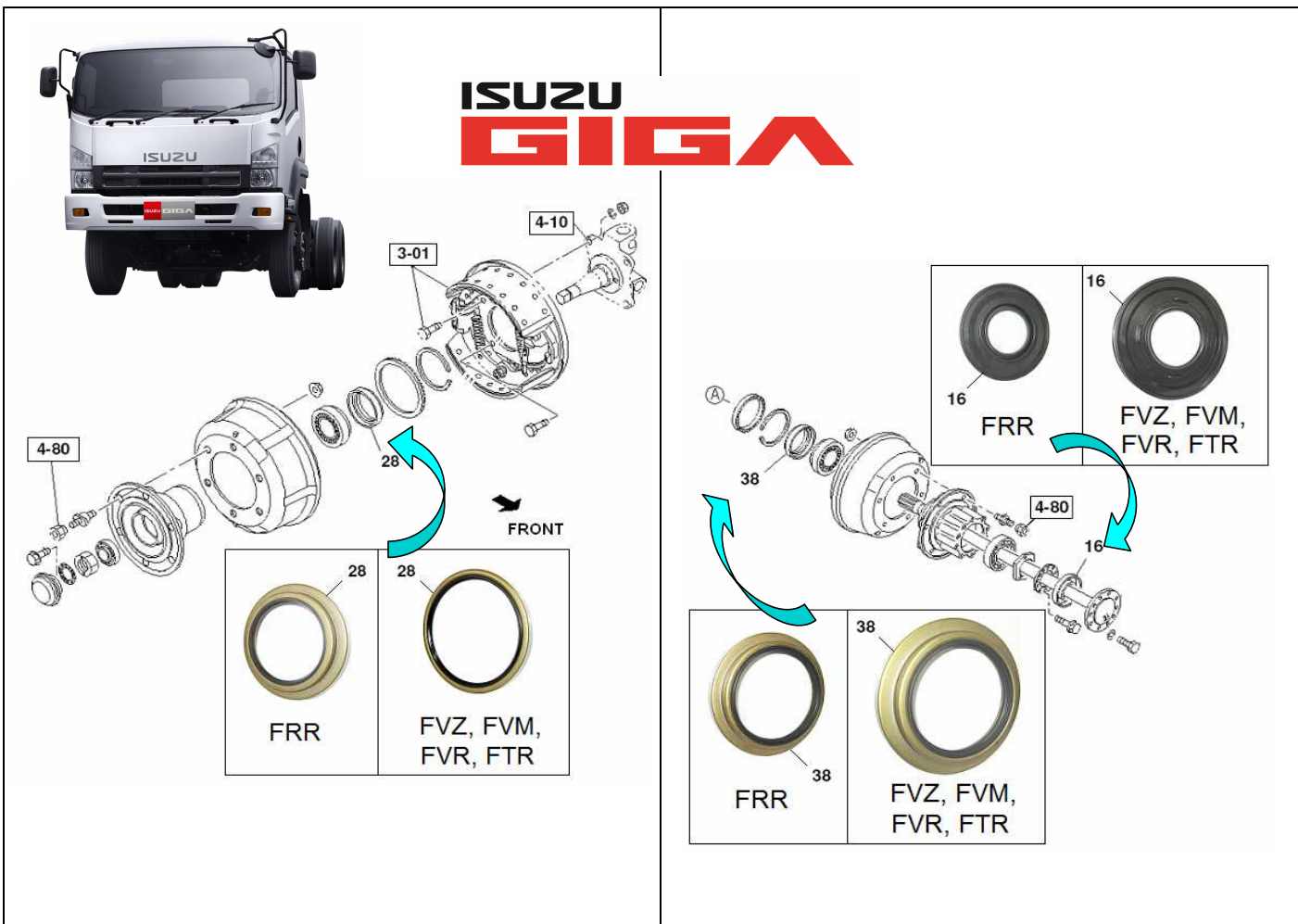
FIG.NO : 4-11 FRONT HUB AND DRUM
