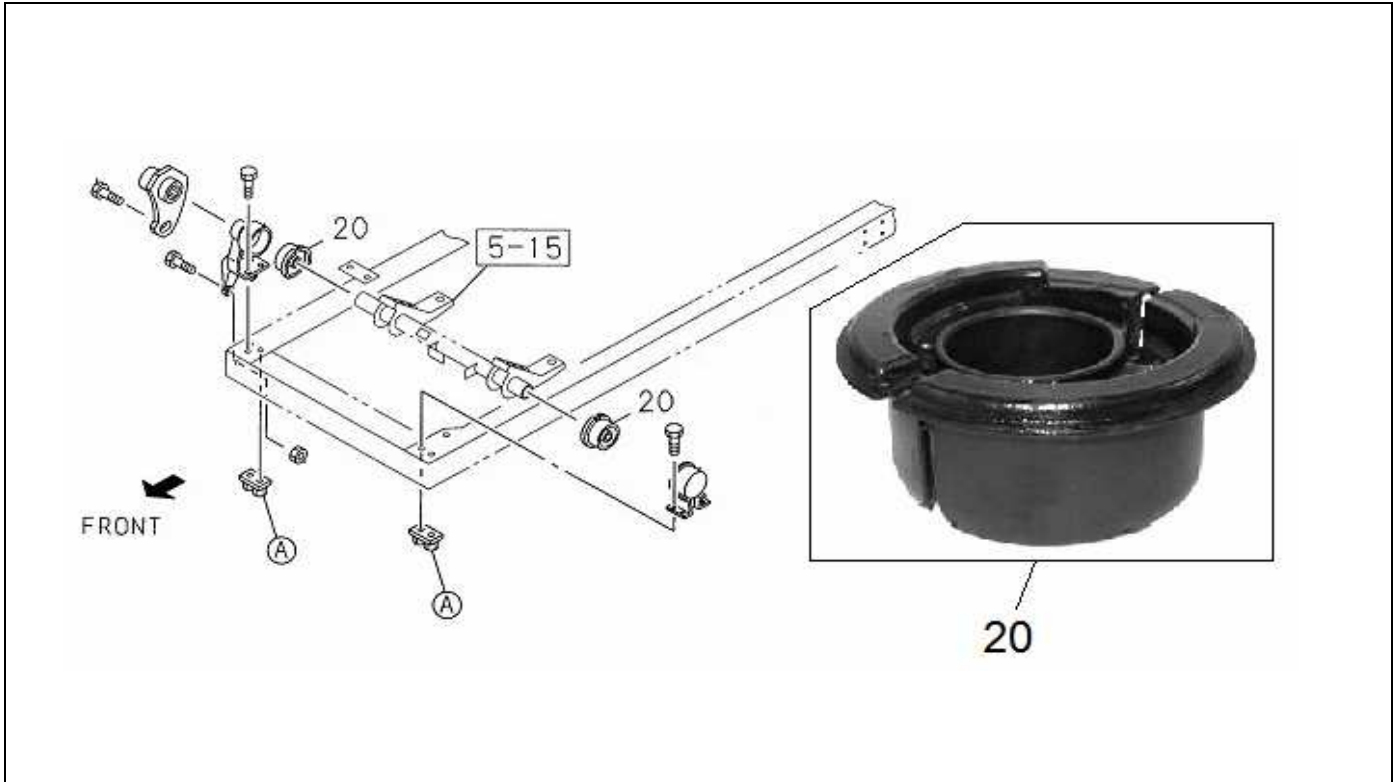
FIG.NO : 5-10 RUBBER MOUNTING CAB BRKT
