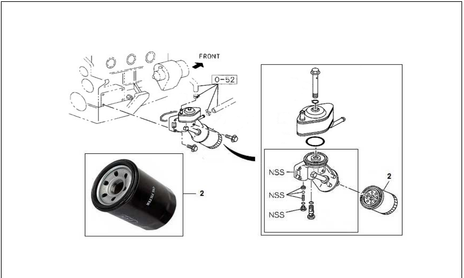
FIG.NO : 0-50 OIL COOLER AND OIL FILTER
