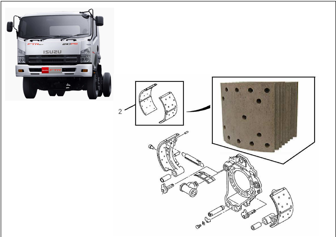
FIG.NO : 3-05 REAR WHEEL BRAKE
