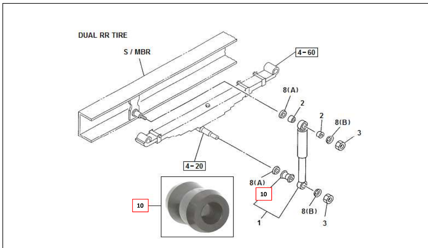
FIG.NO : 4-61 SHOCK ABSORBER; REAR SUSPENSION
