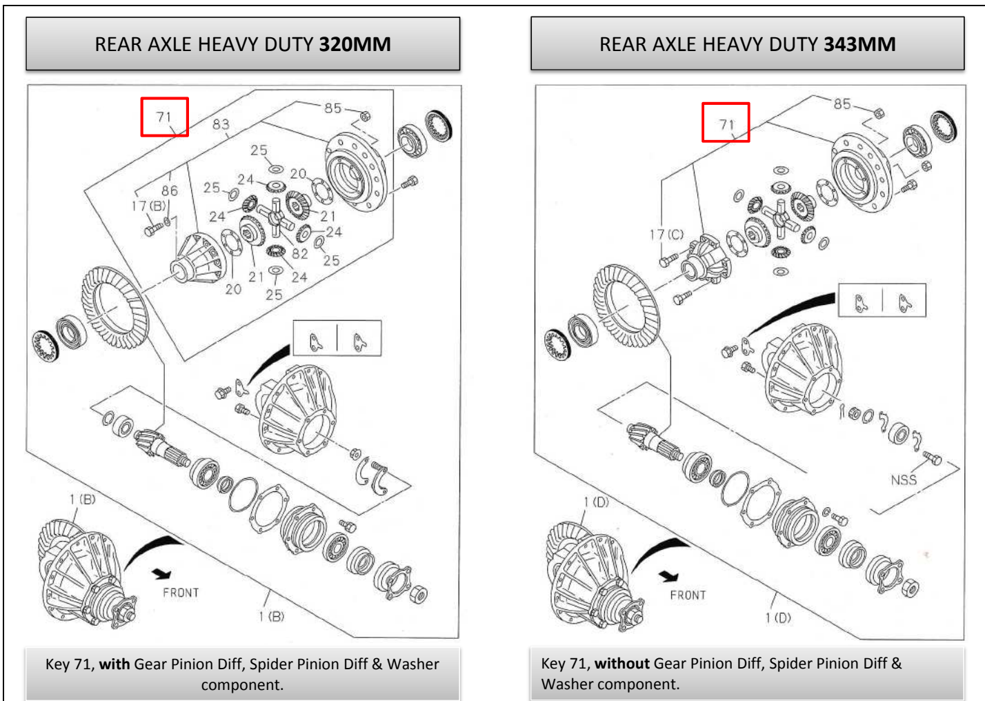
FIG NO : 4-25 REAR FINAL DRIVE
