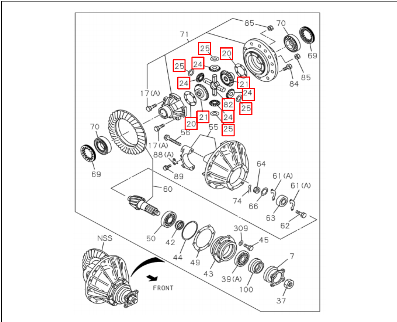
FIG NO : 4-25 REAR FINAL DRIVE
