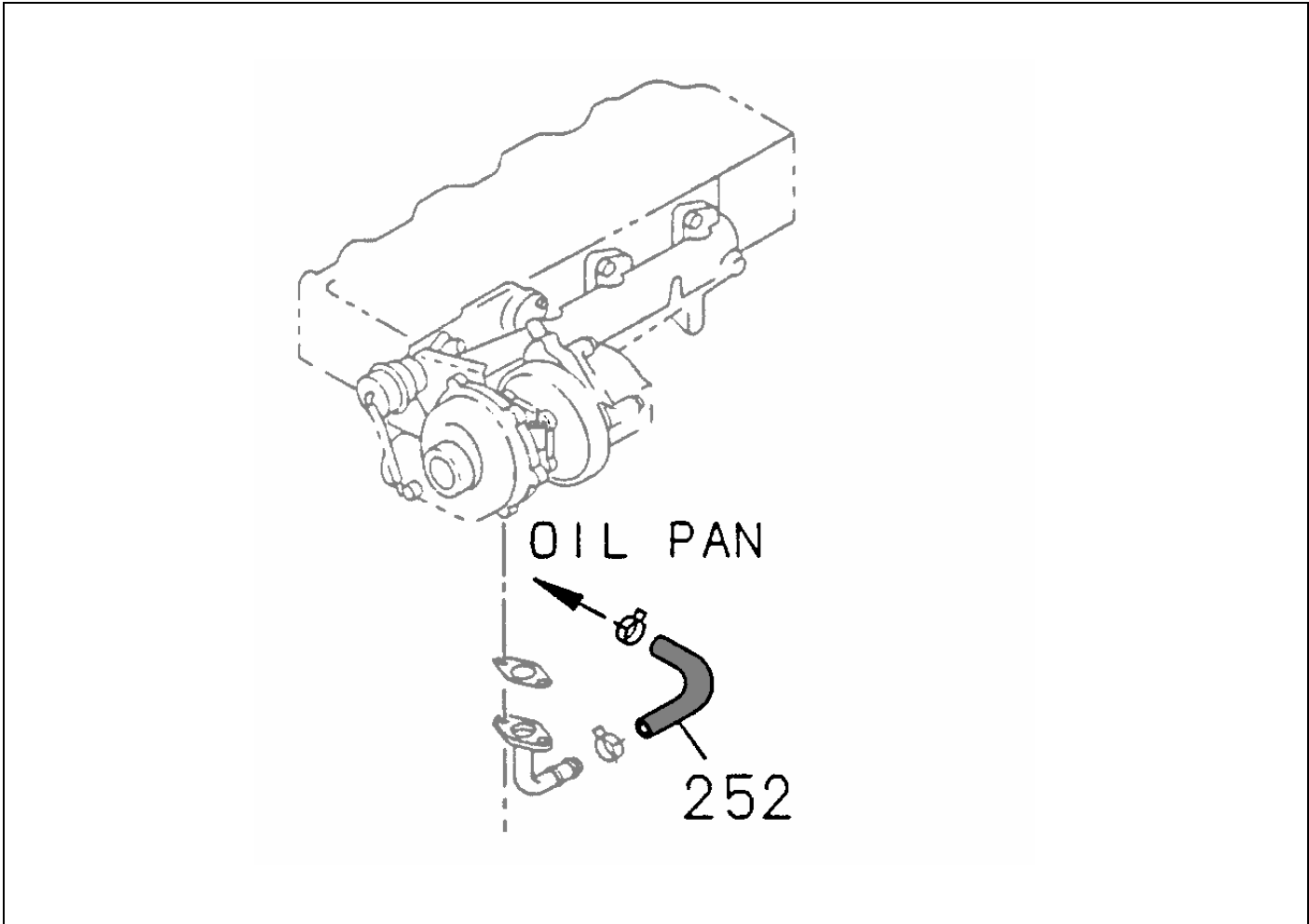
FIG.NO : 0-52 OIL AND VACCUM PIPING; ENGINE
