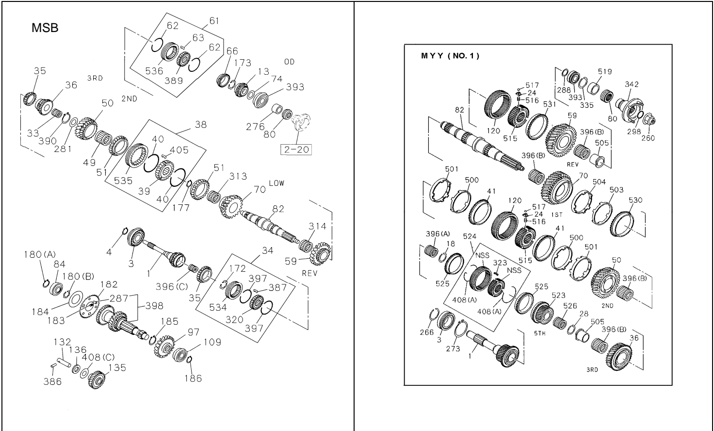
FIG.NO : 2-26 MANUAL TRANSMISSION GEAR
