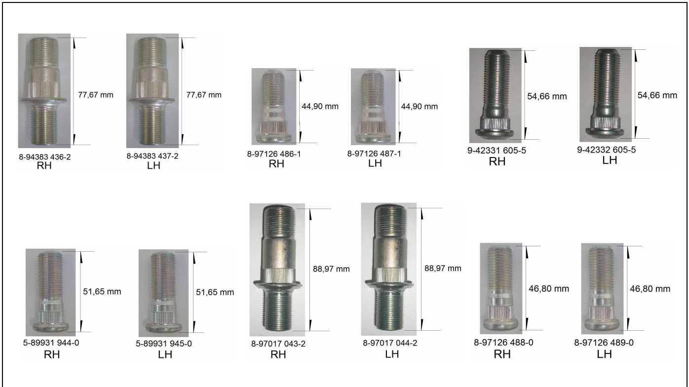
FIG.NO : 4-11 & 4-20 PIN WHEEL
