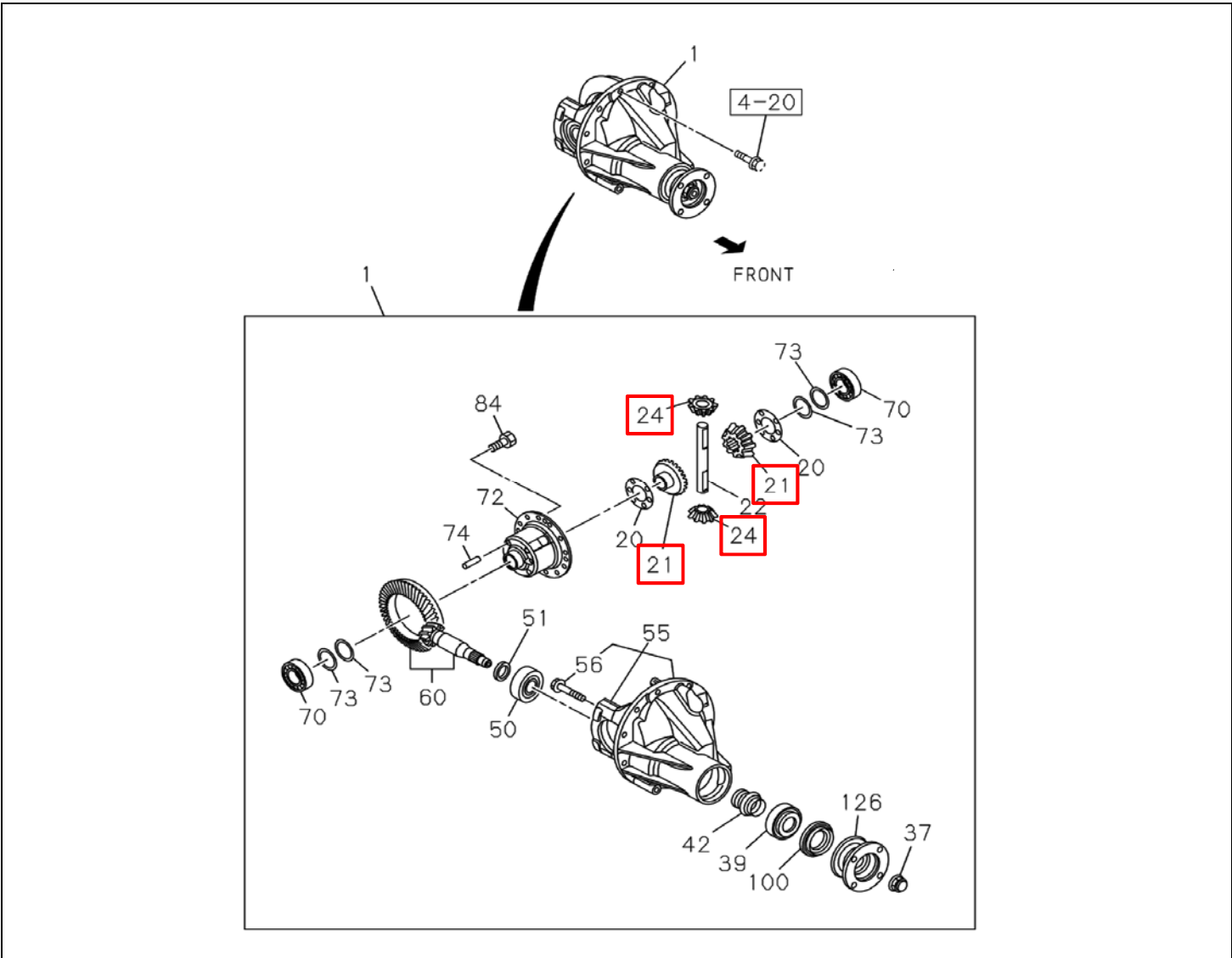
FIG NO : 4-25 REAR FINAL DRIVE
