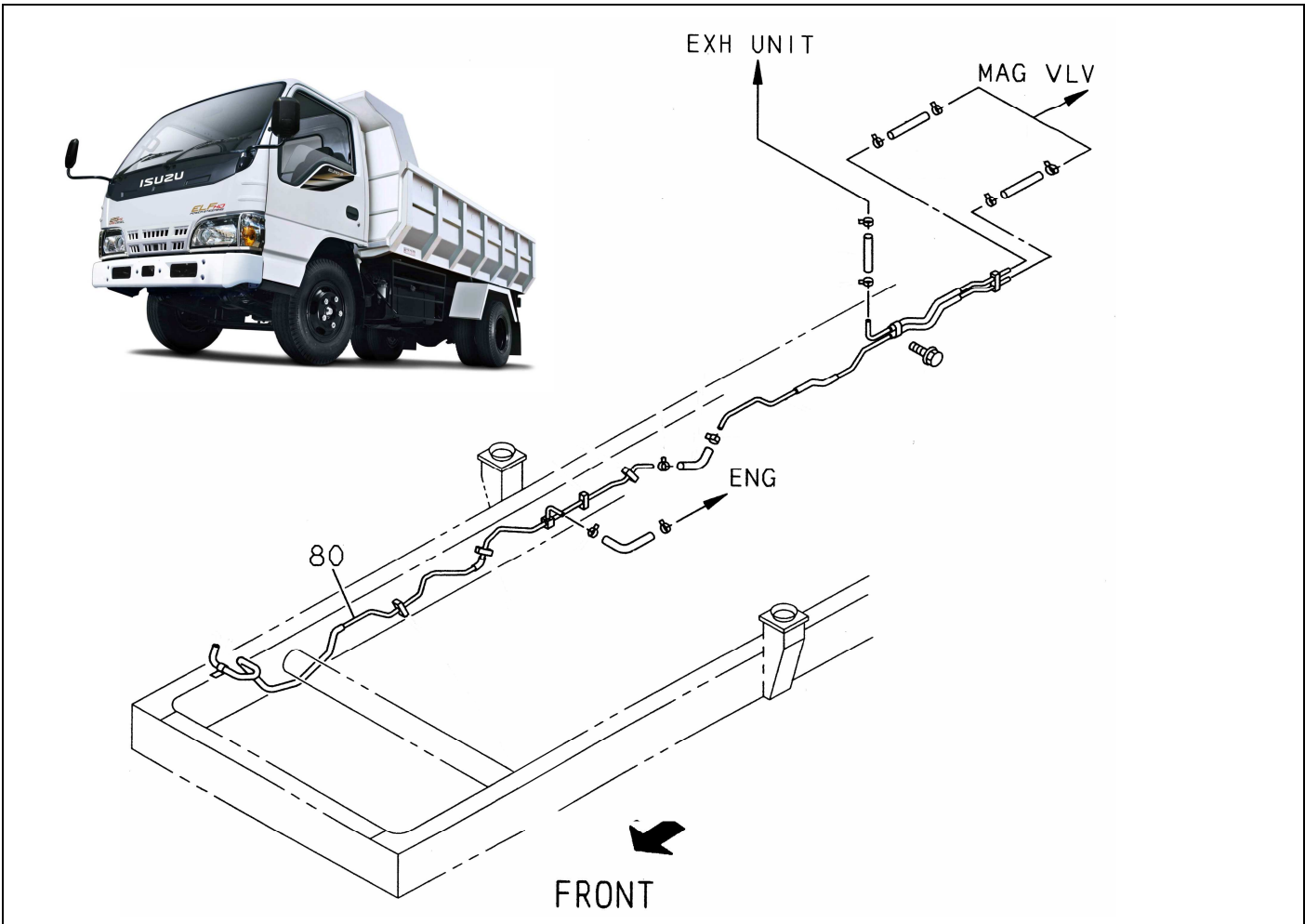
FIG.NO : 3-60 BRAKE PIPING ; VACUUM
