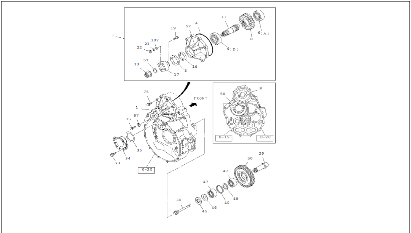
FIG.NO : 0-90 POWER TAKE OFF; FLYWHEEL
