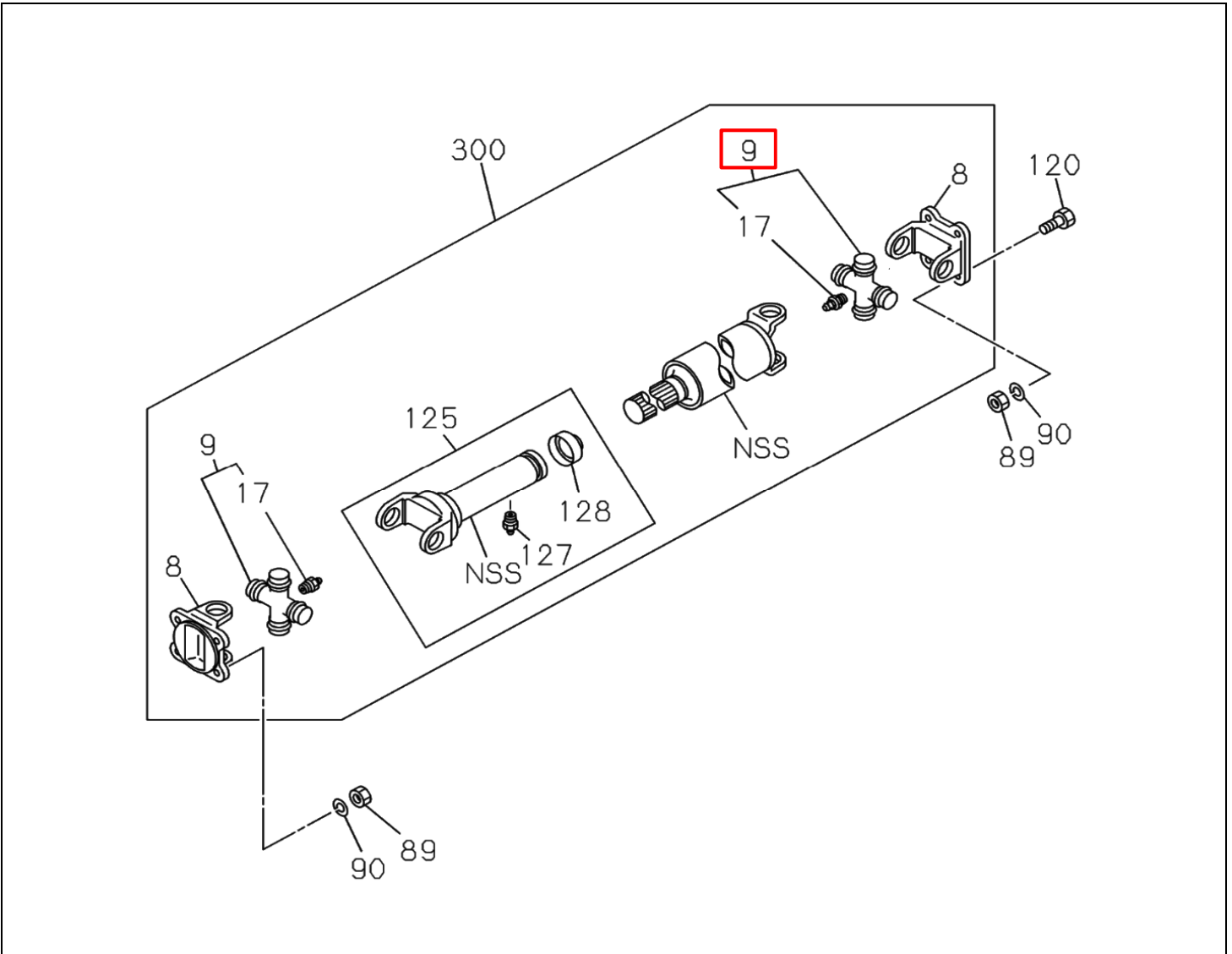
FIG NO : 4-01 PROPELLER SHAFT
