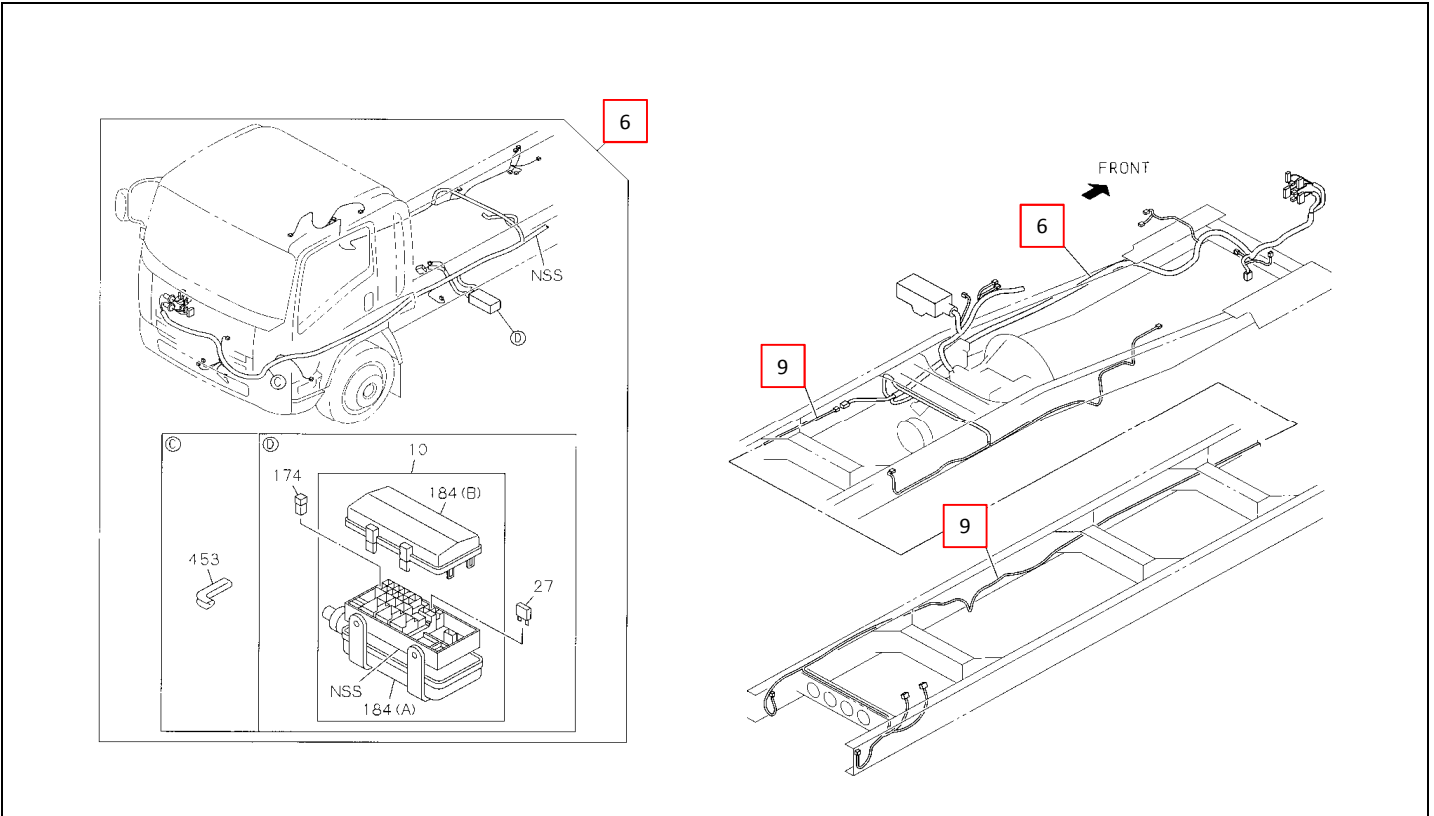
FIG.NO : 8-10 WIRING HARNESS AND FUSE
