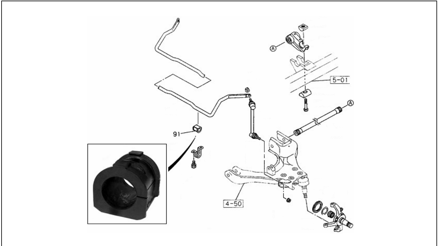
FIG.NO : 4-10 BUSHING STABILIZER
