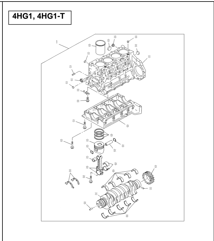
FIG.NO : 0-01 PARTIAL ENGINE
