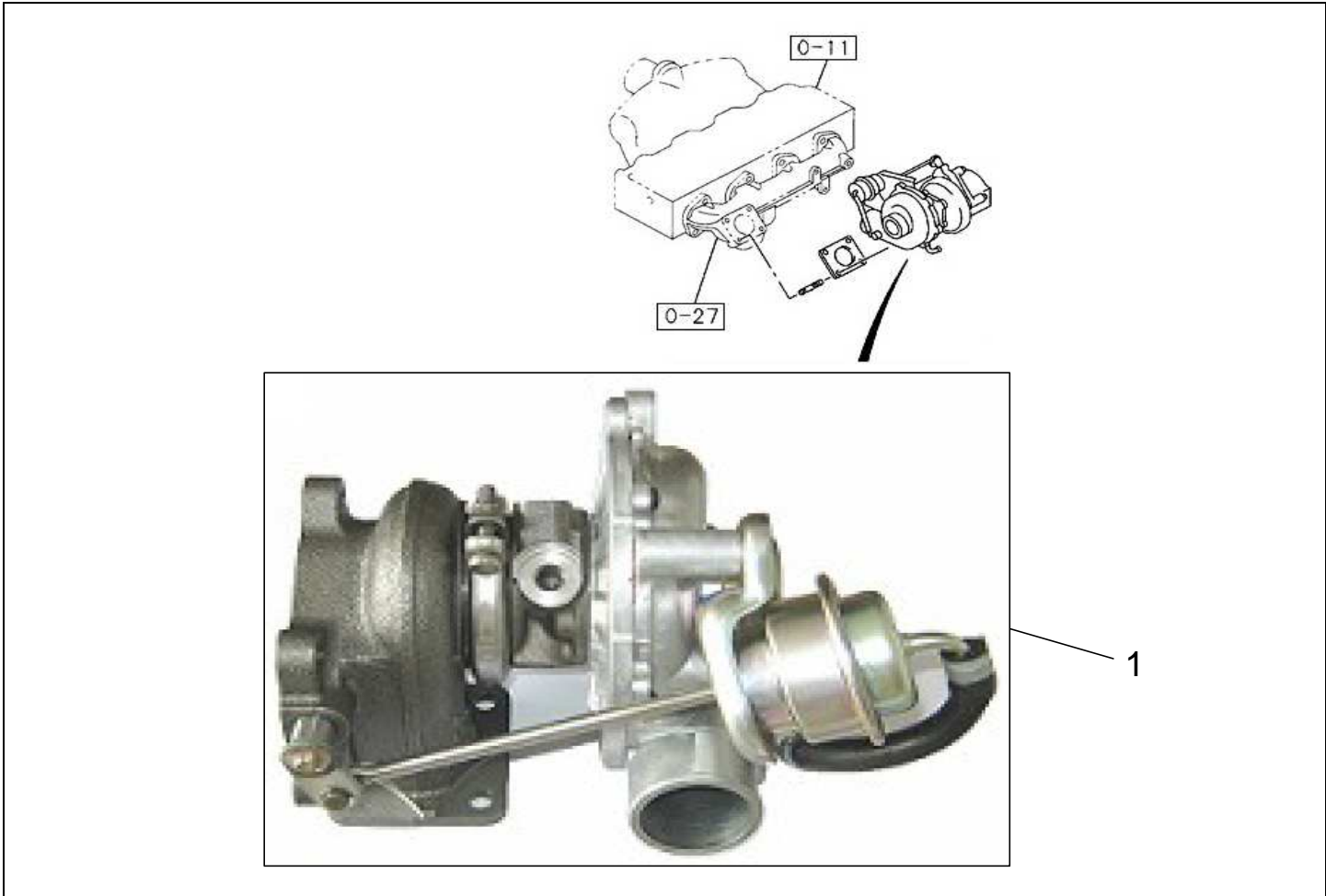
FIG.NO : 0-36 TURBOCHARGER
