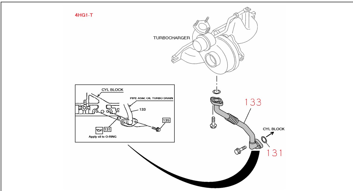
FIG.NO : 0-36 TURBOCHARGER SYSTEM
