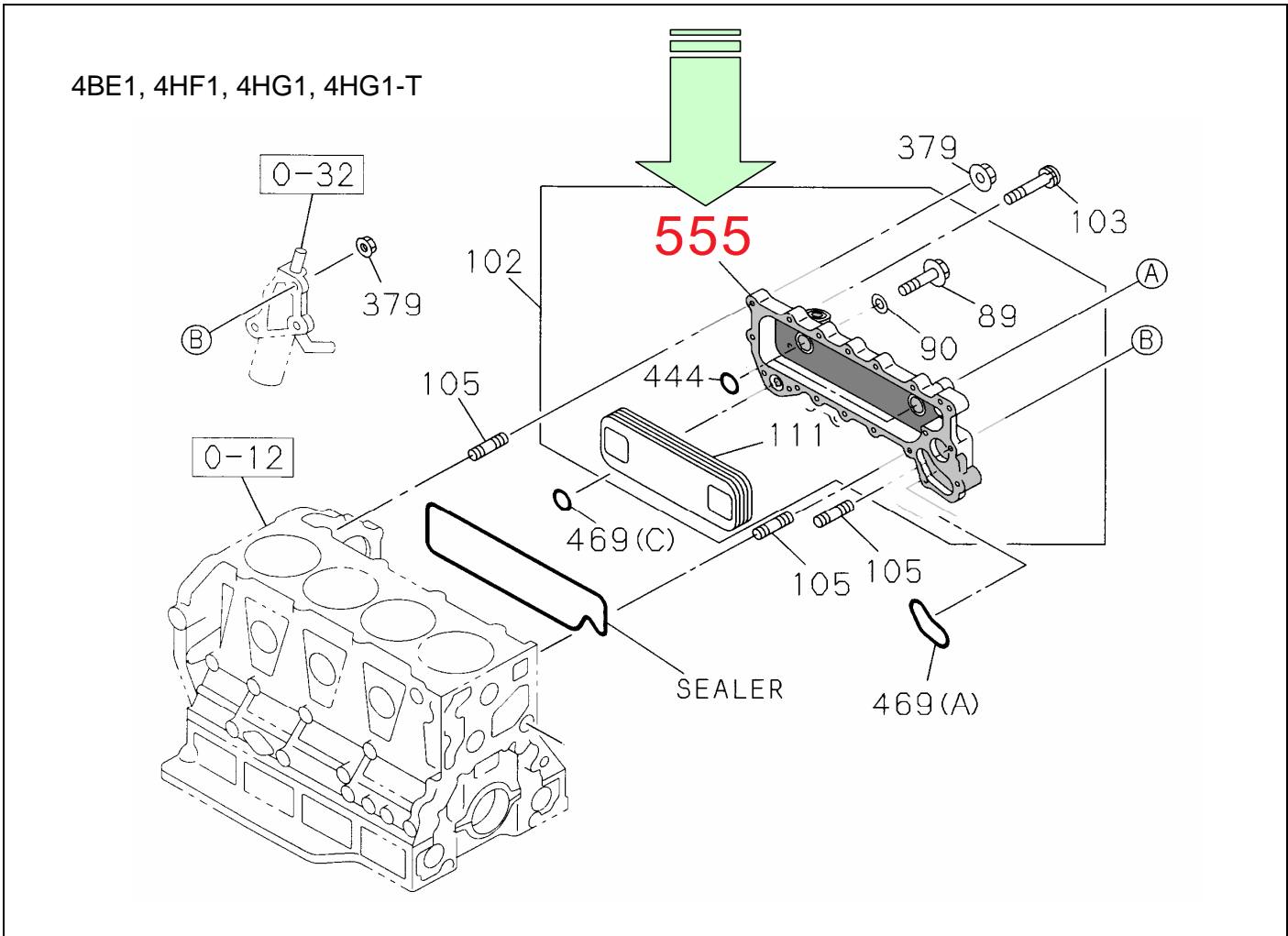
FIG.NO : 0-50 OIL COOLER AND FILTER
