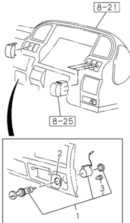
FIG.NO : 8-26 ELECTRICAL CONTROL AND OTHER PARTS
