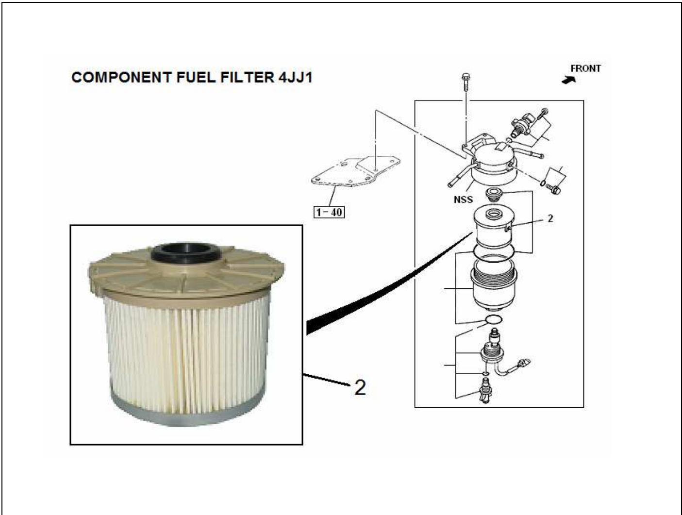
FIG.NO : 0-41 FUEL FILTER AND BRACKET
