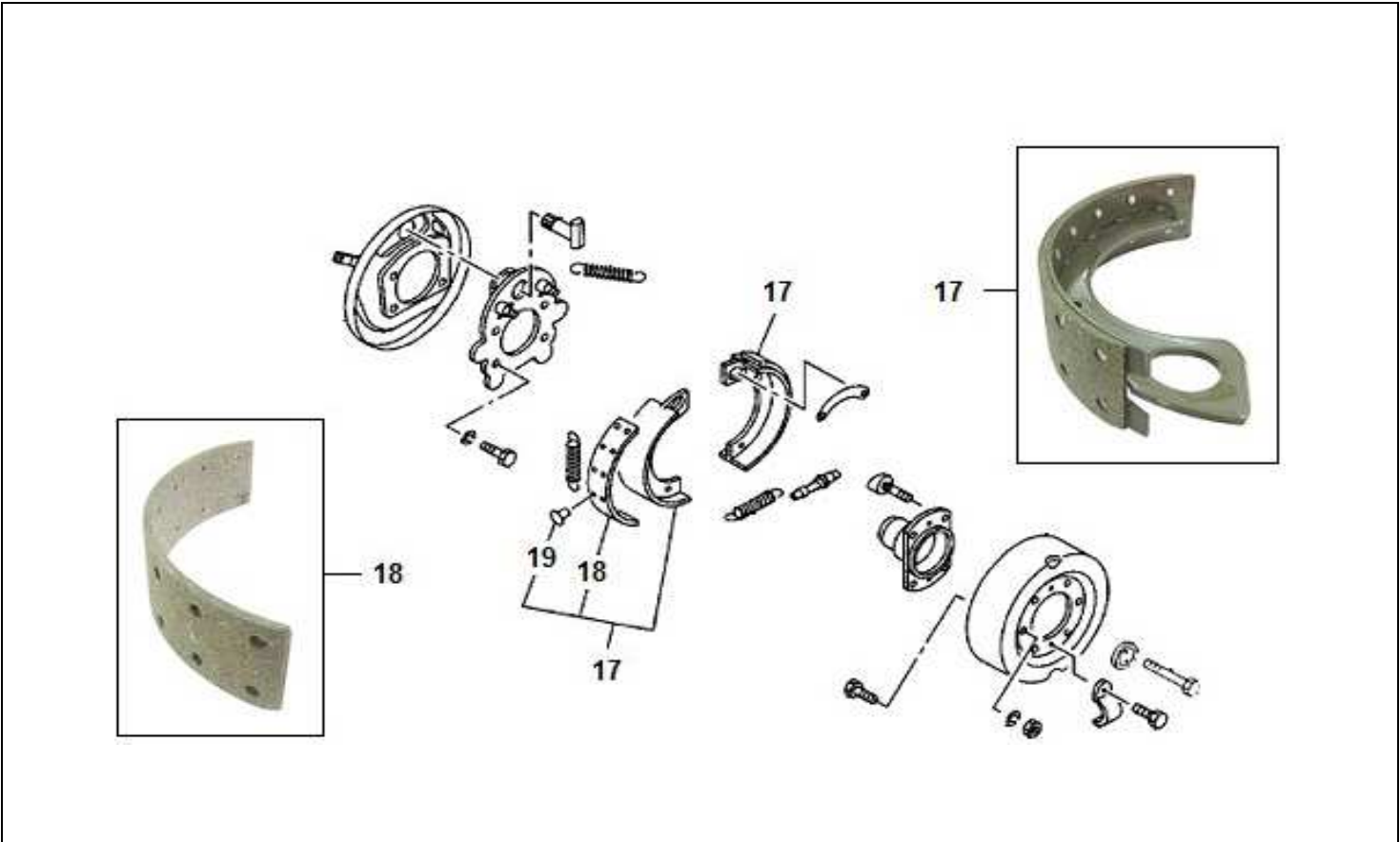
FIG.NO : 3-08 PARKING BRAKE
