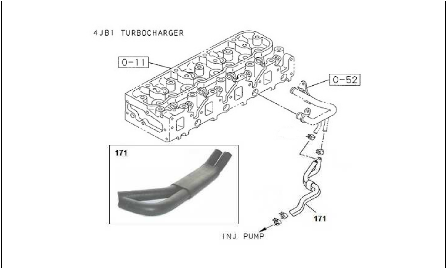
FIG.NO : 0-32 WATER PIPING; ENGINE
