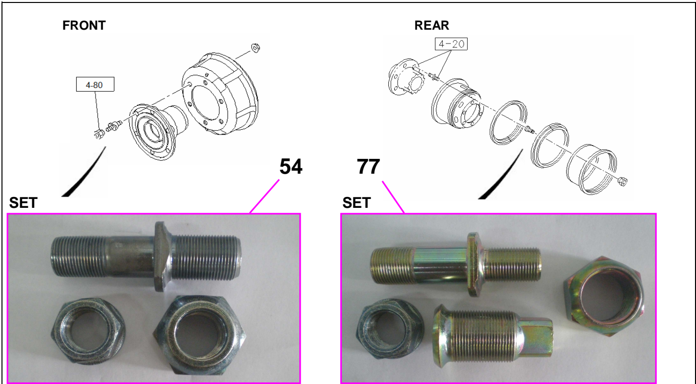
FIG.NO : 4-11 FRONT HUB & 4-20 REAR AXLE
