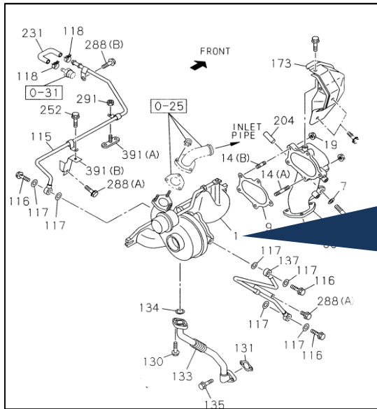
FIG.NO : 0-36 TURBOCHARGER SYSTEM
