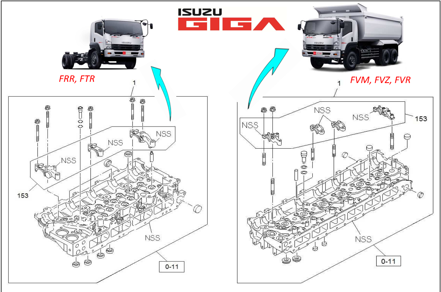
FIG.NO : 0-11 CYLINDER HEAD
