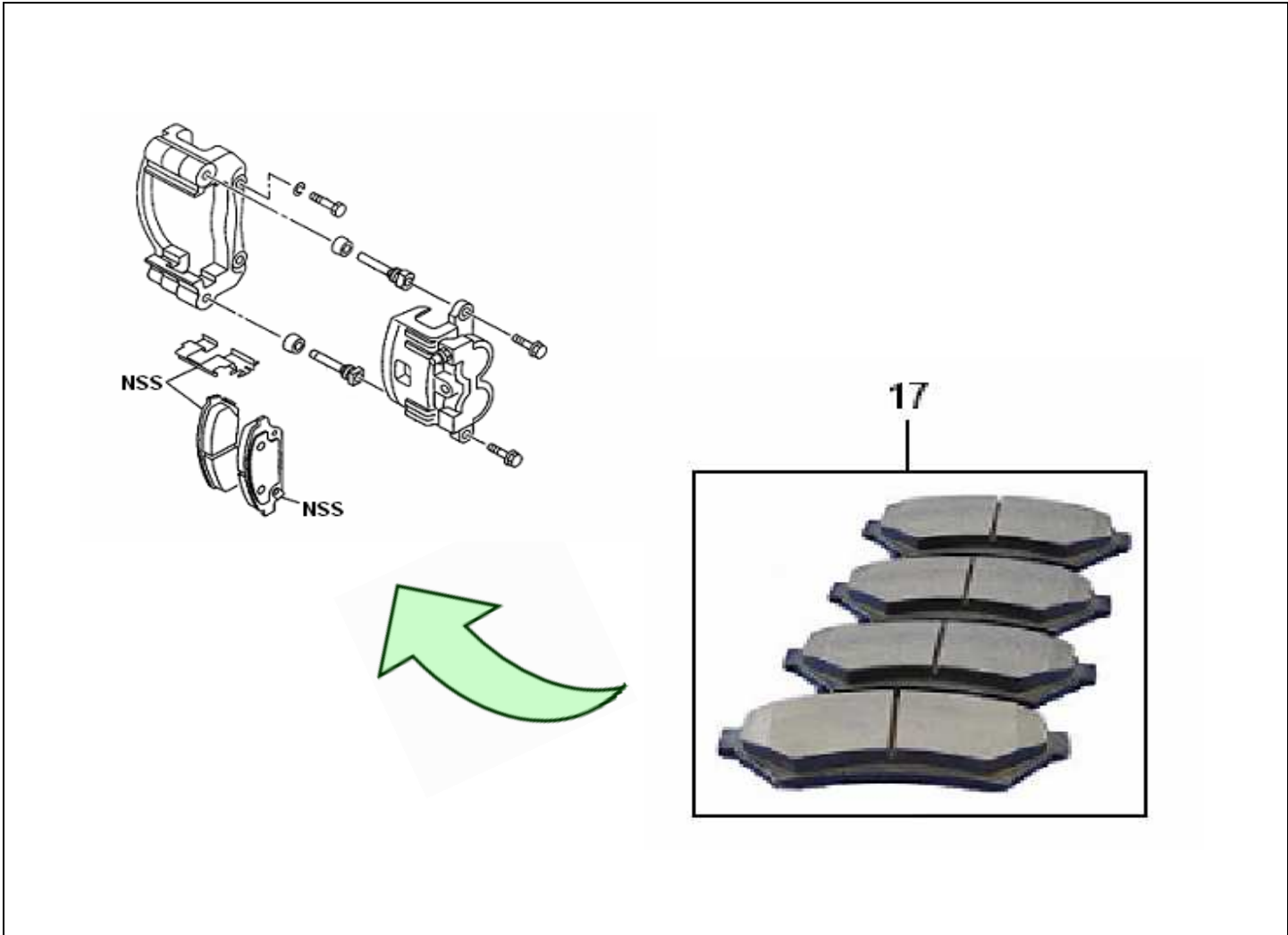
FIG.NO : 3-02 FRONT DISC BRAKE CALIPER
