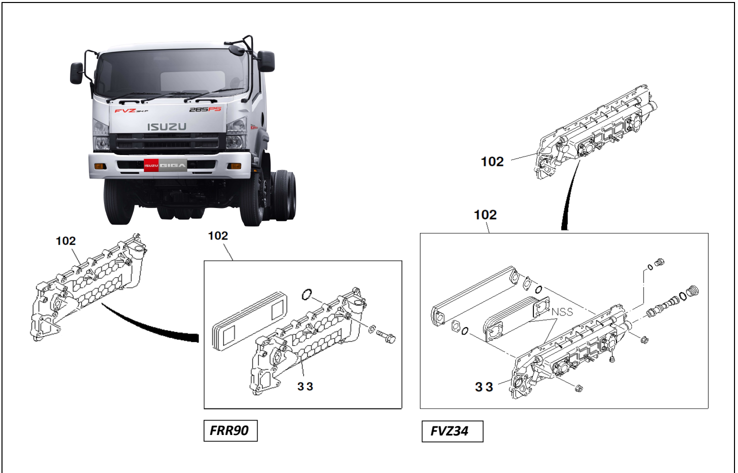
FIG.NO : 0-50 OIL COOLER AND OIL FILTER
