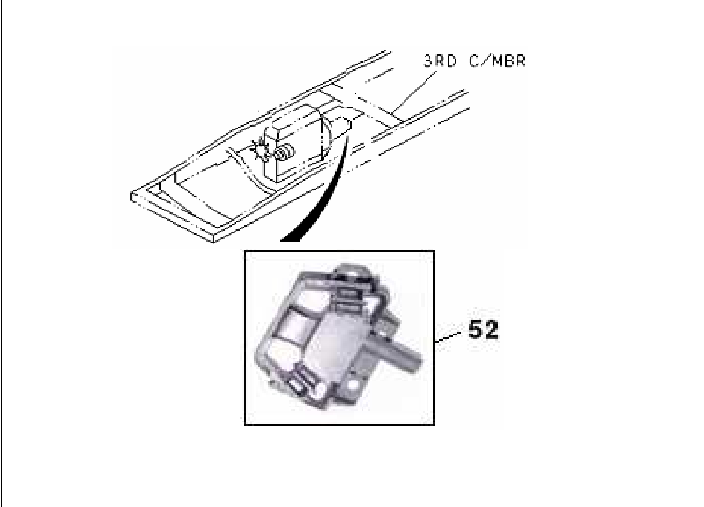
FIG.NO : 0-22 ENGINE MOUNTING
