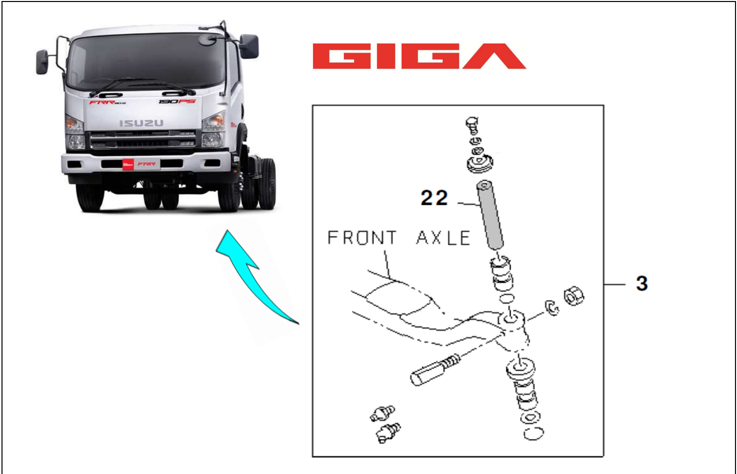
FIG.NO : 4-10 FRONT AXLE
