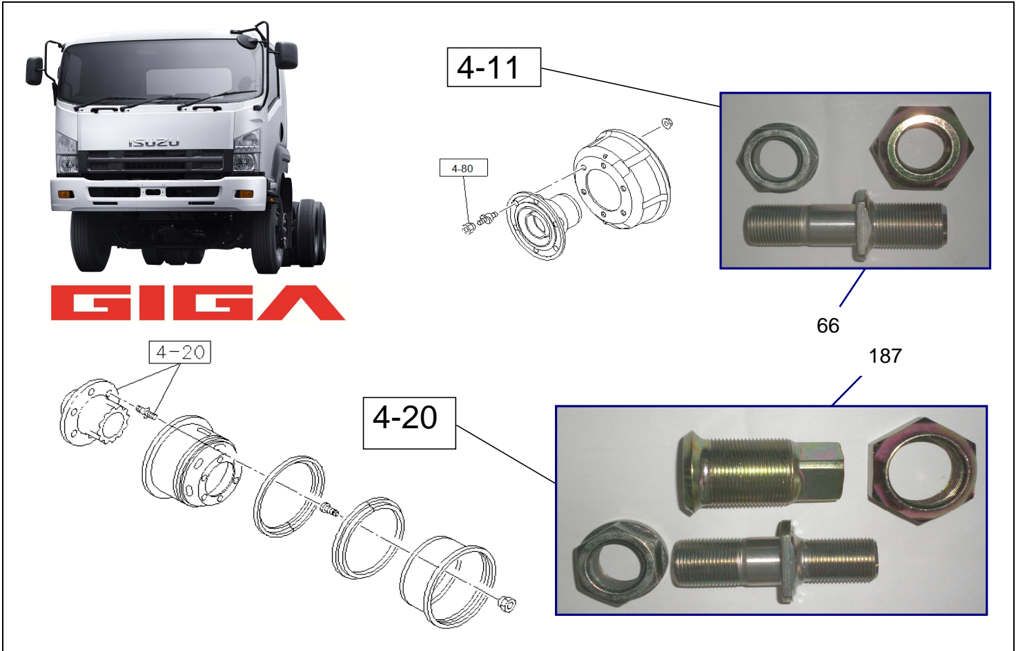
FIG.NO : 4-11 FRONT HUB AND DRUM & 4-20 REAR AXLE
