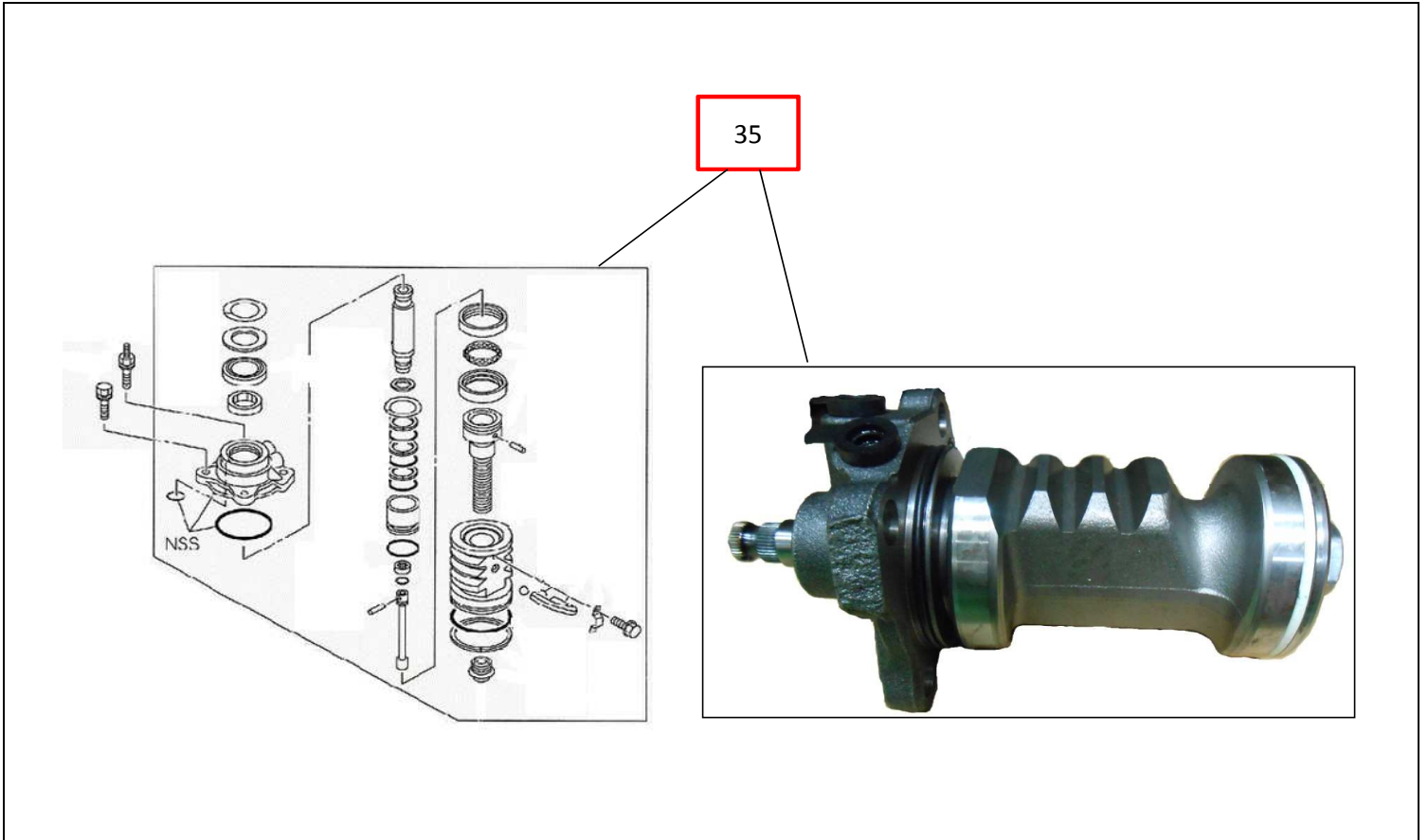
FIG.NO : 4-40 STEERING UNIT
