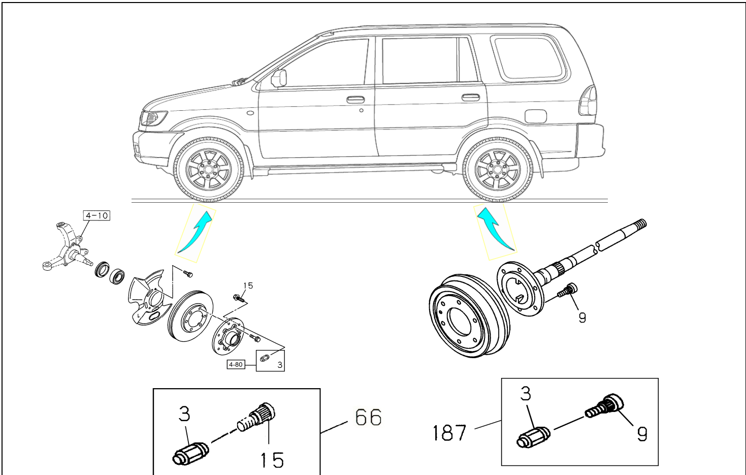
FIG.NO : 4-11 FRONT ROTOR & 4-20 REAR AXLE
